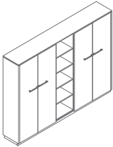
X5129 2496 / 421 / 1871 291.3 kg
