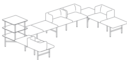
AR22 3630 / 1810 / 910 68.38 kg
